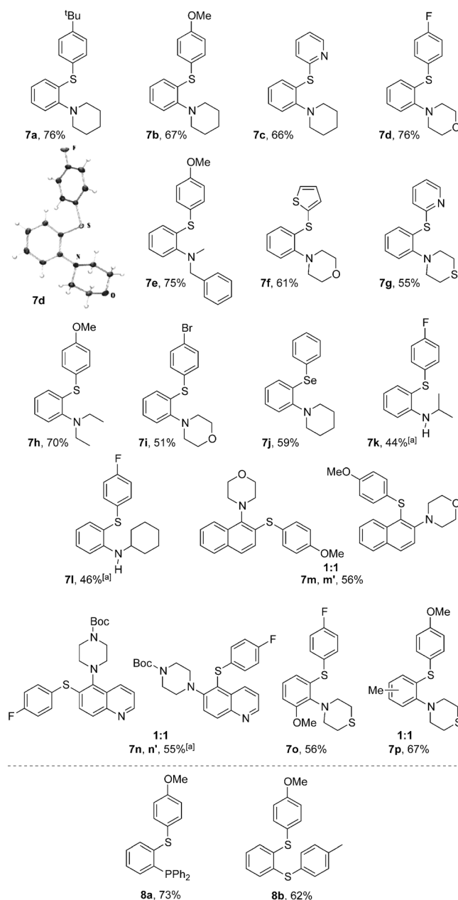
Figure 1. Scope of the (2-aminophenyl)benzothioether substrate. Reaction conditions: thiol (1 mmol), t PrMgCl (2.2 mmol), and aryne precursor (1.2 mmol) were stirred at –78 °C for 45 min, then warmed to 0 °C. The resulting intermediate Grignard was quenched with 1.5 mol of R 1 R 2 N–OBz in the presence of CuCl (10 mol%) and phenanthroline (10 mol%; see SI). [a] An additional zincation step was performed by adding ZnCl 2 (0.5 equiv) after the initial thiolate addition. The thermal ellipsoids of the X-ray structure of 7d were set at 50%. [19]
